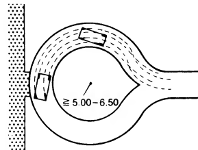
3 Car turning circle radius for an entrance drive \geq 5-6.50 m
